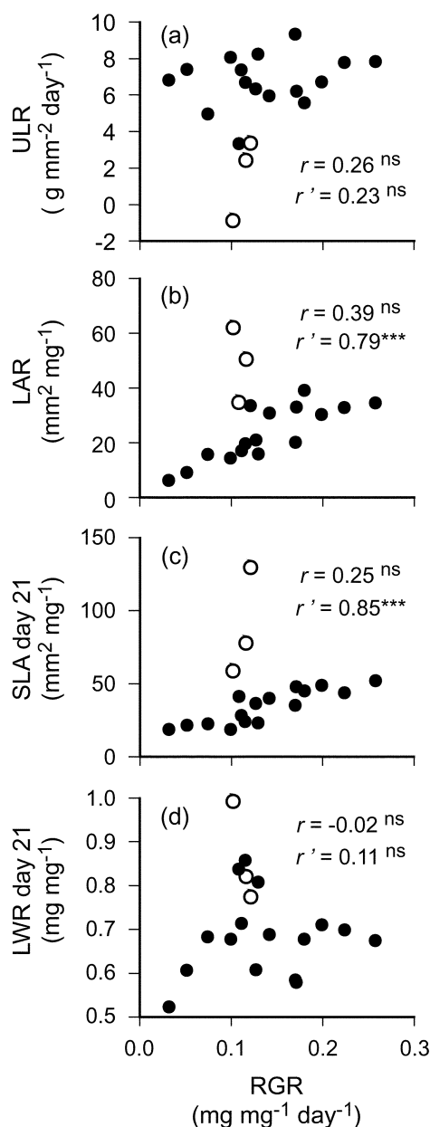
Figure 4. Correlations between relative growth rate (RGR) of bog plant seedlings and (a) unit leaf rate (ULR), (b) overall leaf area ratio (LAR), (c) specific leaf area at day 21 (SLA) and (d) leaf weight ratio at day 21 (LWR). Correlations coefficients are given for the entire data set ( r ) and without the three smallest-seeded species ( r' ), which are shown by hollow circles. Significance of correlations: ns, not significant; * P \leq 0.05 ; ** P \leq 0.01 ; *** P \leq 0.001 . P values were adjusted using the stepwise Bonferroni procedure based on k = 4 tests.
