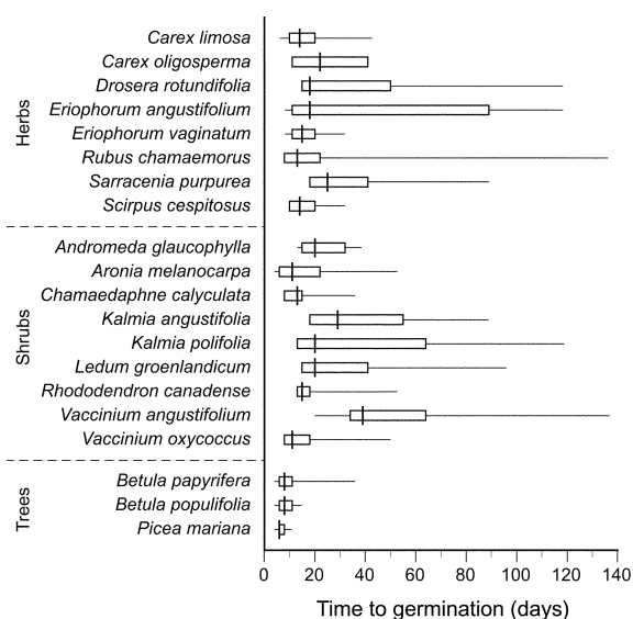
Figure 1. Germination timing of surface-sown seed of herbaceous, shrub and tree species. Horizontal lines show initial and final germination, boxes show 10% and 90% germination and the vertical line shows 50% germination.
