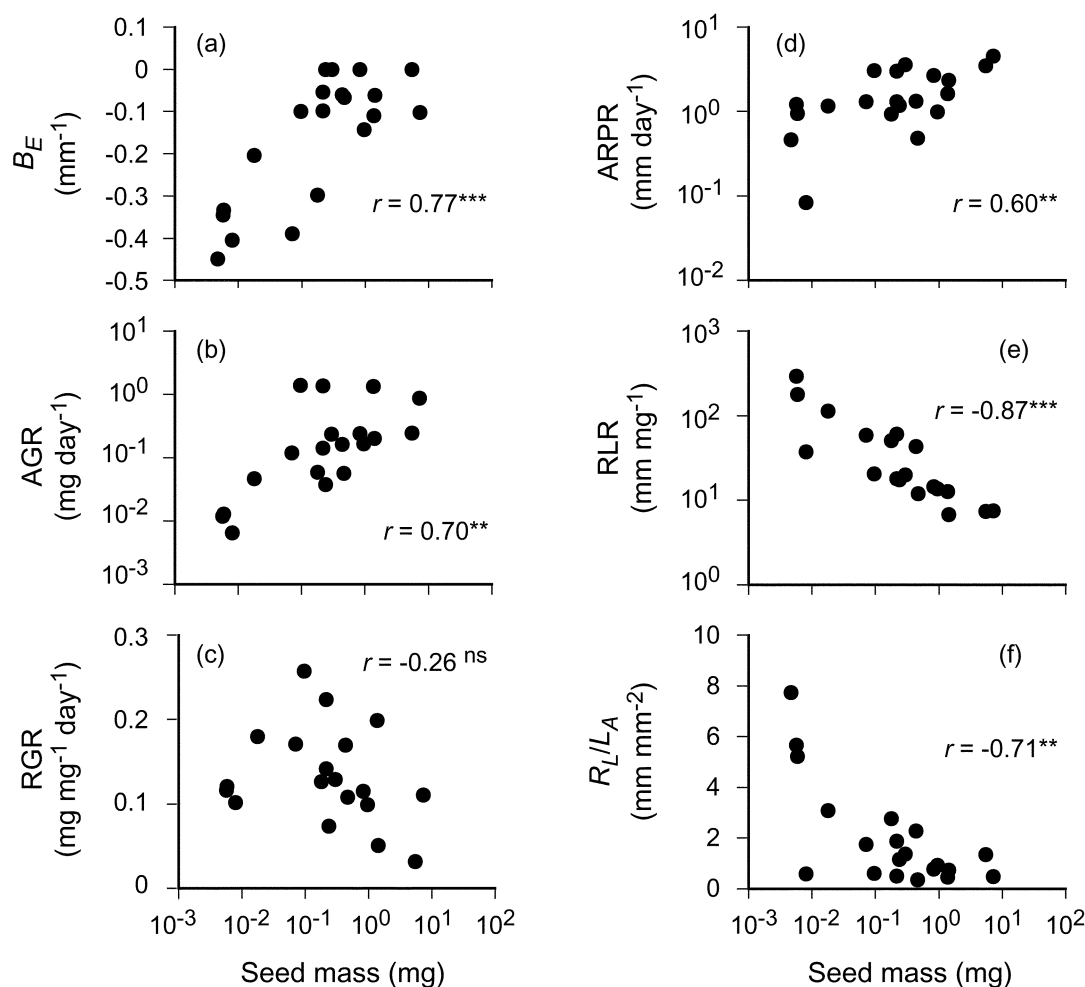
Figure 3. Correlations between log seed mass of bog plants and (a) the slope of the negative exponential functions of seed emergence versus burial ( B_E ), (b) seedling absolute growth rate (AGR, log scale), (c) seedling relative growth rate (RGR), (d) absolute rate of root penetration (ARPR, log scale), (e) overall root length ratio (RLR, log scale), and (f) the ratio of maximum root length to leaf area ( R_L/L_A ). Significance of correlations: ns, not significant; * P \leq 0.05 ; ** P \leq 0.01 ; *** P \leq 0.001 . P values were adjusted using the stepwise Bonferroni procedure based on k = 6 tests.
