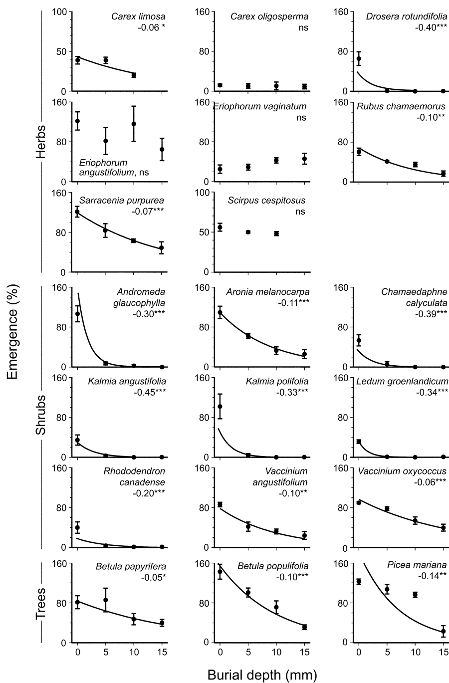
Figure 2. Seedling emergence of study species as functions of seed burial depth (mean \pm SE). Emergence is expressed as percent of viable seed sown, corrected using separate seed viability tests, except for Carex limosa and Scirpus cespitosus , which are expressed as percent seed sown. Percent emergence occasionally have values in excess of 100% as a result of seed viability corrections. Curves are fitted to species with significant negative exponential functions between mean emergence and burial depth. Values of significant slopes are given below the species name. Significance of slopes: ns, not significant; * P \leq 0.05 ; ** P \leq 0.01 ; *** P \leq 0.001 .
